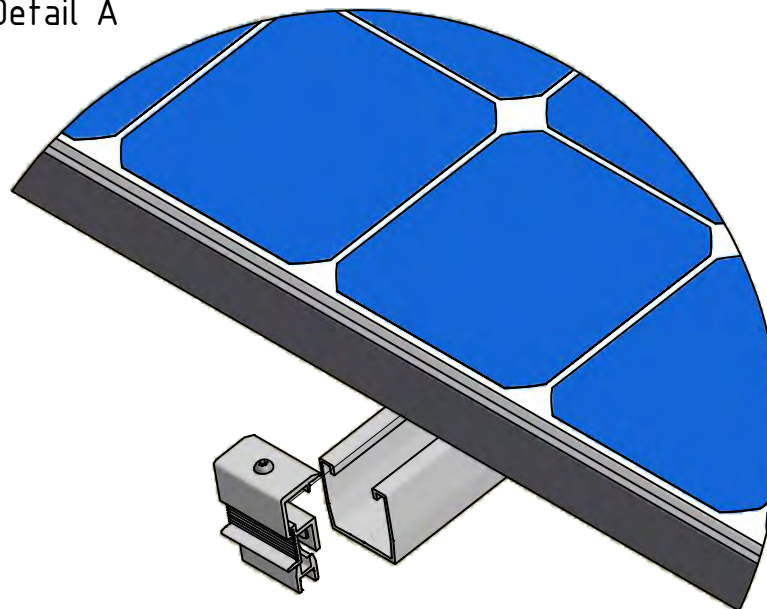
Detail A
