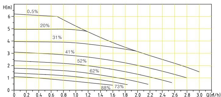
Signal CPA-E55/xx-xxx S PWM
