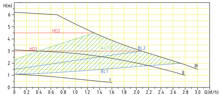
CPA-E55/xx-xxx circulation pump
