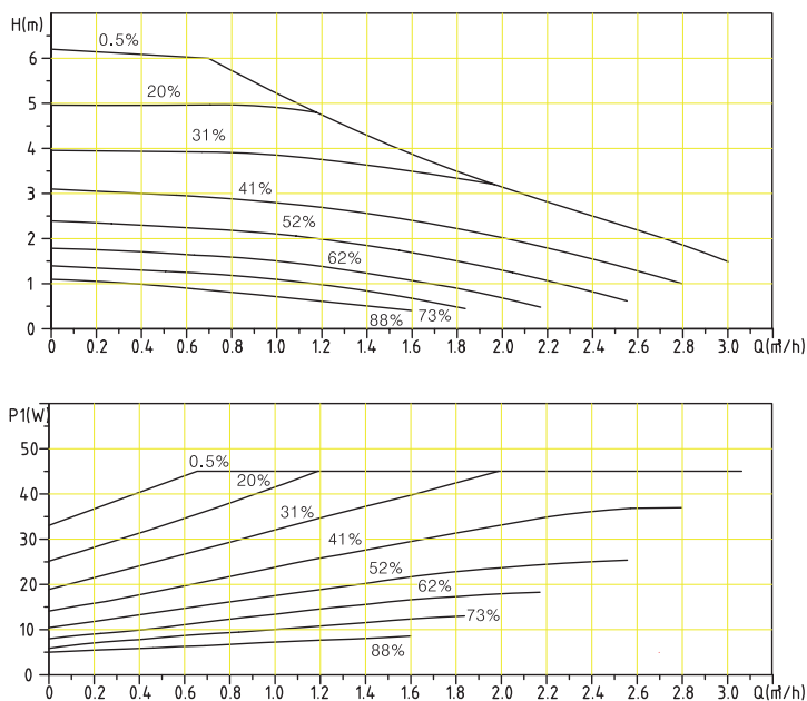
CPA-E55/× ×-xxx S PWM Signal
