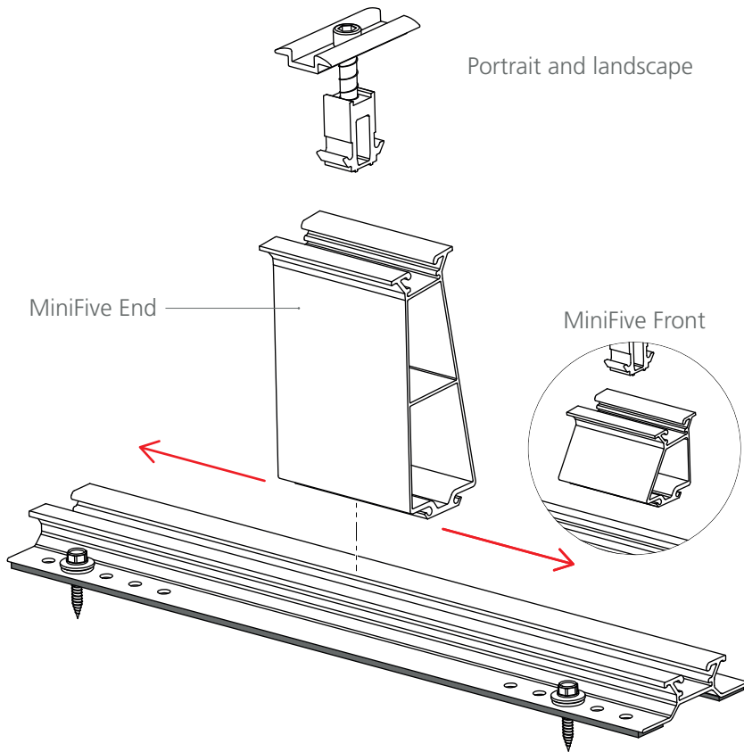
MiniFive Front 5/9 cm
