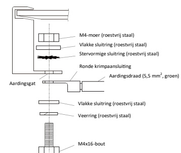
Figuur 6. Aardingsmethode
