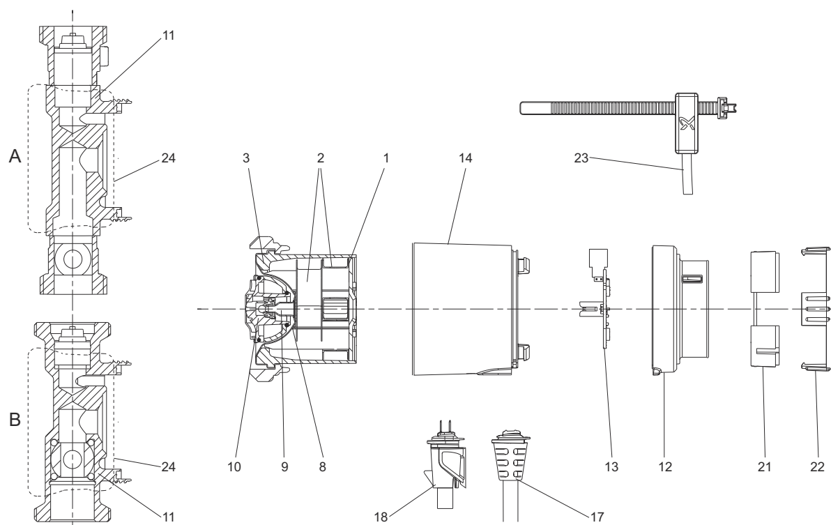
Fig. 20 Sectional drawing of COMFORT PM
